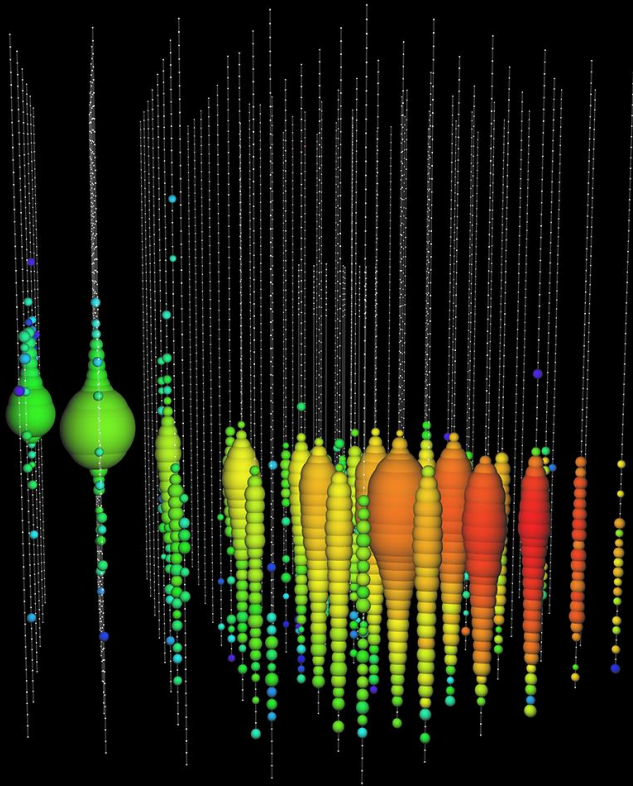
Example of IceCube detected event
